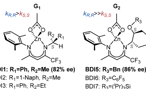
Scheme 2 Structures of G 1 and G 2 generations of zinc β-diimine catalysts for enantioselective ROCOP of CHO and CO 2 . 12d
