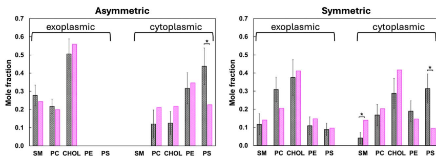
Fig. 2 The mole fraction of lipids in each class in the first solvation shell in the exoplasmic and cytoplasmic leaflets, and in the asymmetric membrane simulation (left panel) and in the symmetric membrane simulation (right panel), averaged over the last 5 \mu s of each trajectory simulations. Gray filled bars are the results for the first solvation shell of the receptor, and the magenta filled bars are the composition of that species averaged over the entire leaflet. An asterisk (*) indicates cases for which the lipid composition of the bulk is outside the 95% confidence interval of its composition in the first shell. The PE class includes plasmalogen.
