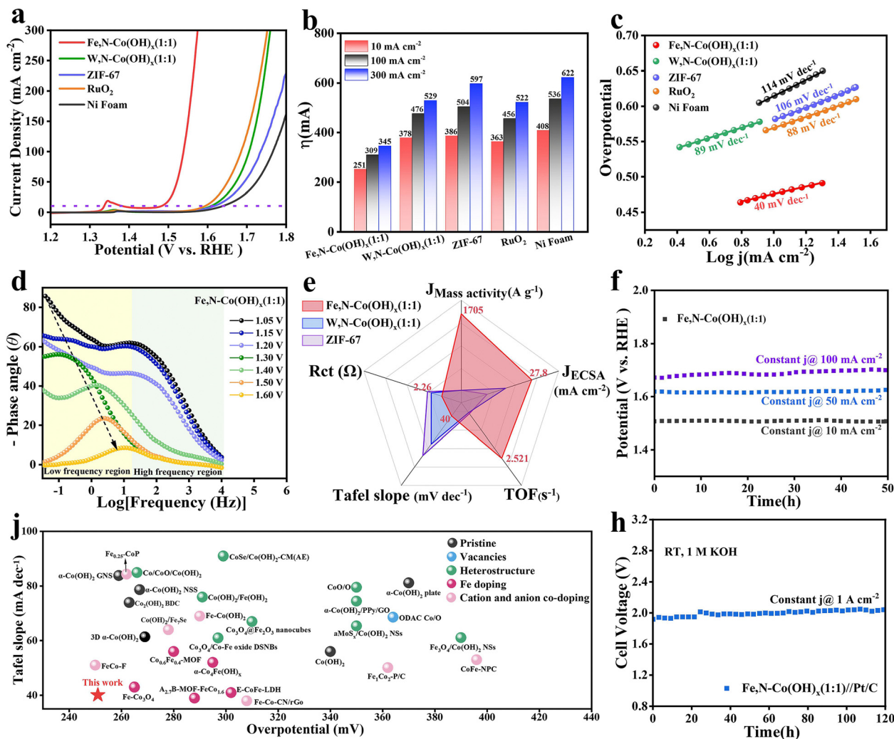
Fig. 3 Electrochemical performance and durability of \text{Fe,N-Co(OH)}_x (1:1) catalyst. (a) LSV polarization curves in 1 M KOH solution at a scan rate of 5 \text{ mV s}^{-1} . (b) Overpotential ( \eta ) at 10, 100, and 300 \text{ mA cm}^{-2} . (c) Tafel slopes for \text{Fe,N-Co(OH)}_x (1:1) during the OER. (d) Bode plots of \text{Fe,N-Co(OH)}_x (1:1) during the OER. (e) Comparison of OER activity between \text{Fe,N-Co(OH)}_x (1:1) (red), \text{W,N-Co(OH)}_x (1:1) (blue), and ZIF-67 (orange-red). (f) Chronopotentiometric curve at 10, 50, and 100 \text{ mA cm}^{-2} . (g) Comparison with recently reported catalysts. (h) The long-term durability of the prepared AEMWEs ( \text{Fe,N-Co(OH)}_x (1:1)//Pt/C) measured at 1 \text{ A cm}^{-2} current density (operated at room temperature at a flow rate of 0.15 \text{ L min}^{-1} ).
