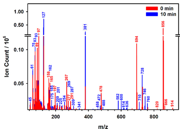
Fig. 4 Electrospray ionization-mass spectrometry (ESI-MS) analysis of experiment with 30 \mu\text{M} iohexol, 3.0 \text{mg L}^{-1} humic acids, and 5.5 \text{mg L}^{-1} \text{ClO}^- at pH 7.0 after (red) 0 and (blue) 10 min irradiation ( \lambda_{\text{cut-off}} \geq 295 nm). The m/z values are labeled in colors corresponding to the spectra with the largest intensity. Each spectrum was corrected by subtracting the corresponding solvent background.
