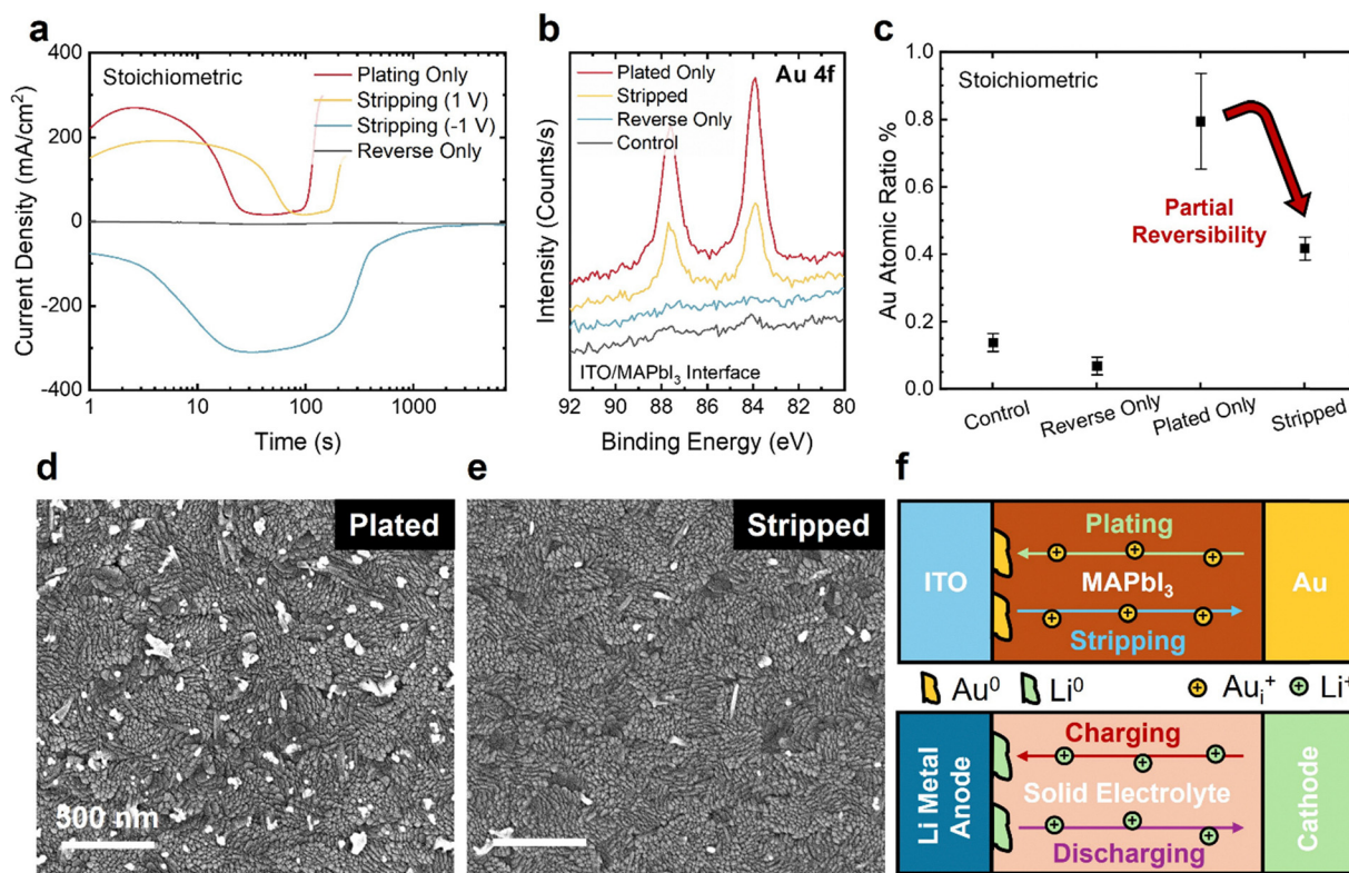
Fig. 3 Partial reversibility of Au migration in ITO/MAPbI 3 /Au devices. (a) J-t characteristics during the Au plating process for the “plated-only” device (1 V, T 3 , red), as well as for the “stripped” device during plating (1 V, T 3 , yellow) and subsequent stripping (-1 V, 2 h, blue). A “reverse-only” device (-1 V, 2 h, gray) is included to show the stability of Au as a cathode. (b) and (c) XPS analysis at the ITO interface after perovskite removal: (b) Au 4f spectra and (c) Au atomic percentages for each biasing condition. (d) and (e) SEM images of accumulated Au 0 at the ITO interface for the (d) “plated-only” and (e) “stripped” pixels. (f) Schematic comparison between our ITO/MAPbI 3 /Au device and a prototypical solid-state battery, highlighting the conceptual similarity between the two. Error bars in (c) reflect the standard deviation of Au atomic percentages measured by XPS.
