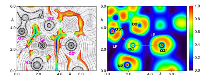
Fig. 5 Left: 2D plot of the Laplacian (dashed lines for negative values and solid lines for positive ones) including the gradient lines (in grey) overlaid with the 2D RDG map for compound Cu 4 L 4 . Right: ELF 2D map of compound Cu 4 L 4 represented in the plane defined by Cu, O2', and O3''. The bond paths are represented as brown lines and BCPs as red dots. The RDG density cut-off is 0.05 a.u. Symmetry operations: '-x, 1/2 - y, z ; ''-1/4 + y, 1/4 - x, 1/4 - z .
