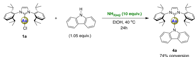
Scheme 5 Synthesis of [\text{Au}(\text{IPr})(\text{cbz})] ( 4a ).
