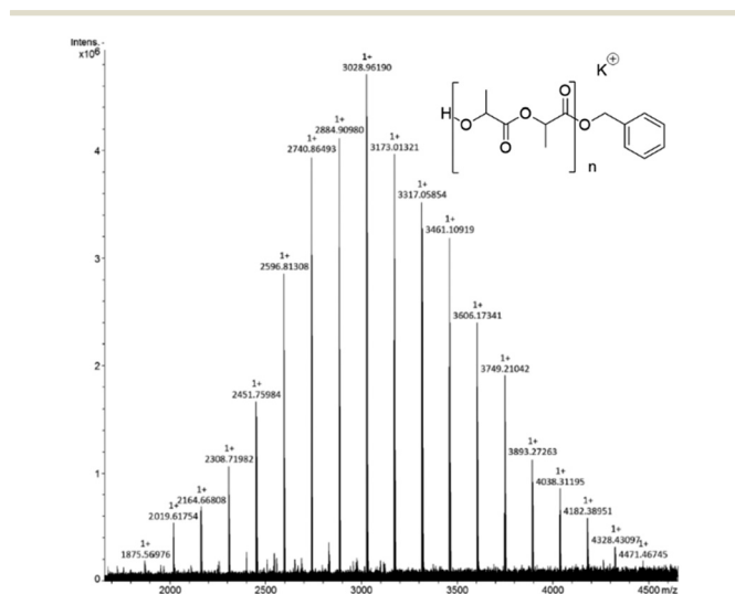
Fig. 4 MALDI-ToF-MS spectrum of PLA obtained with 20 equivalents of L-LA under reaction conditions described in run 1.
