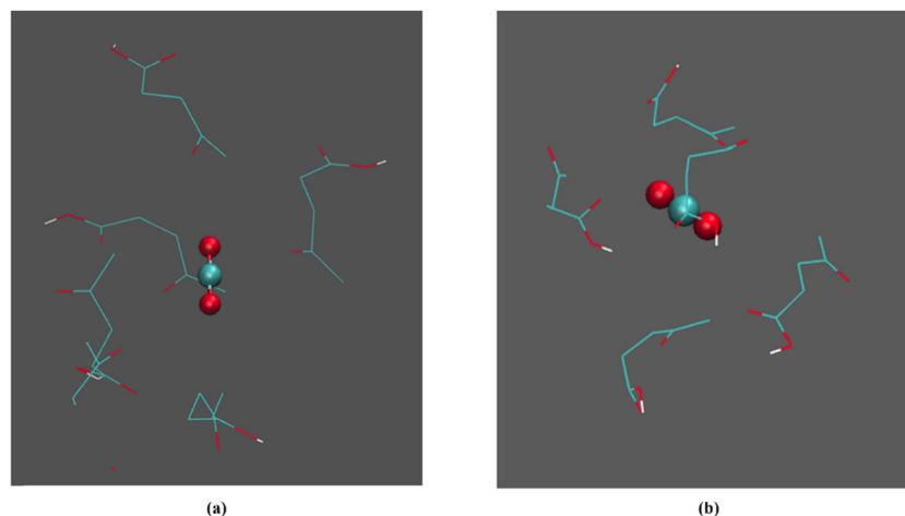
Fig. 5 VMD snapshots (a) and (b)) from our simulation show the levulinic acid molecules in the local environment around \text{CO}_2 [levulinic acid molecules are graphically represented as lines and the atoms in the \text{CO}_2 molecule are shown as spheres. Blue denotes carbon or carbon containing united atoms, red represents oxygen, and hydrogen is shown in white].
