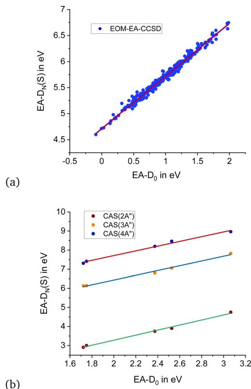
Fig. 9 (a) Correlation plot between EA-D N (S) and EA-D 0 at the EOM-EA-CCSD level. Linear regression gives: y = 1.0106x + 4.7116 with R^2 = 0.9848 . (b) Correlation plots between EA of the three resonances 2 2 A'', 3 2 A'', 4 2 A'' vs. 1 2 A'' (EA-D 0 ) at the CASSCF level. Linear regression gives: 2 2 A'': y = 1.3245x + 0.6306 with R^2 = 0.9948 ; 3 2 A'': y = 1.2473x + 3.9387 with R^2 = 0.9915 ; 4 2 A'': y = 1.2401x + 5.2333 with R^2 = 0.991 . All values are obtained from the orbital stabilization method.
