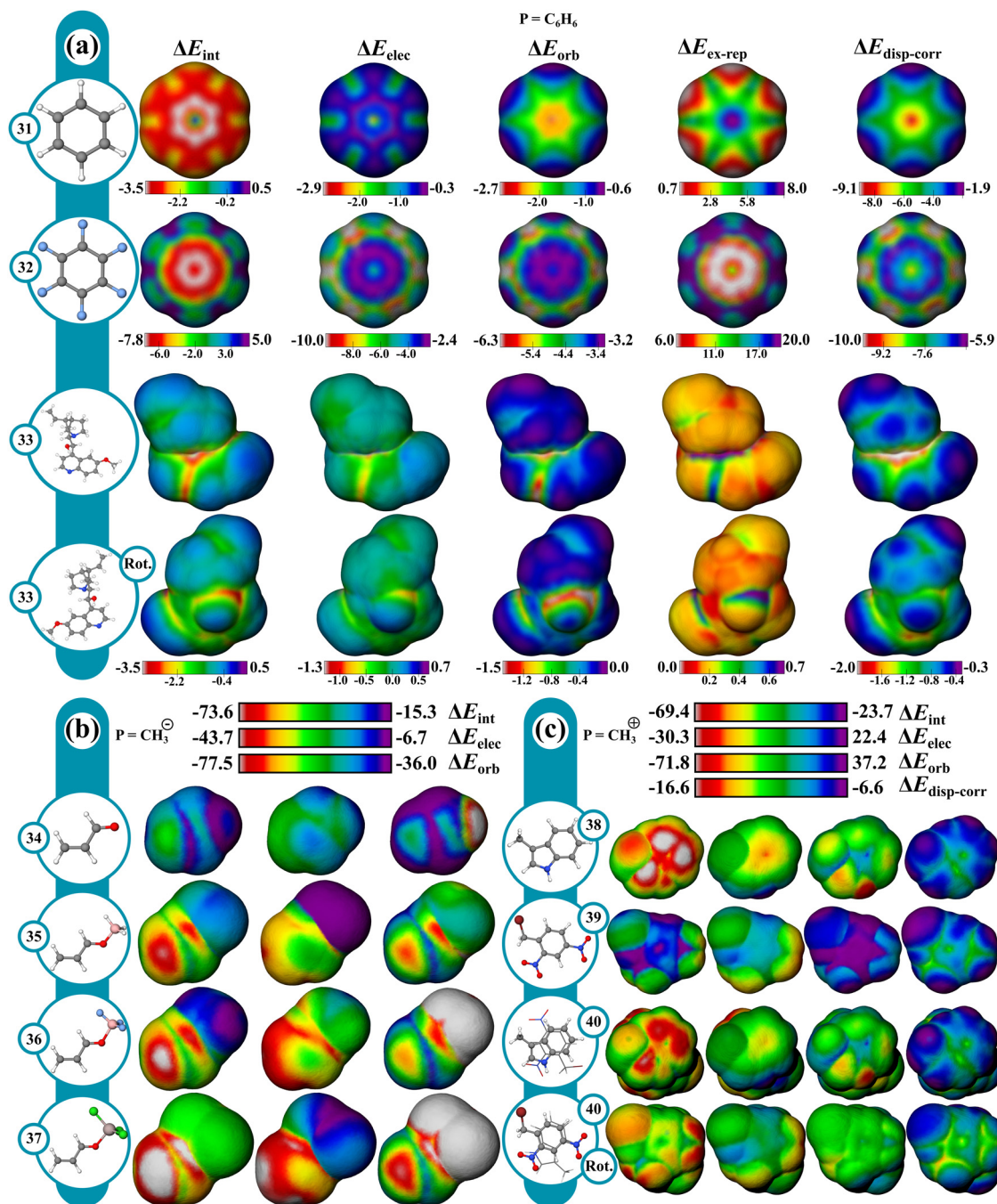
Fig. 7 IMIPs: (a) benzene, hexafluorobenzene, cinchona alkaloid (probe = C_6H_6 ); (b) acrolein, -BH_3 , -BF_3 , and -AlCl_3 coordinated acrolein (probe = CH_3^+ ); (c) methylinole, 2,4-dinitrobenzyl bromide, EDA complex (probe = CH_3^+ ). Isodensity: benzene, cinchona alkaloids, hexafluorobenzene (method B; 1.00 \times 10^{-6} ), acrolein systems (method B; 6.00 \times 10^{-5} ), and EDA complex (method B; 6.00 \times 10^{-5} ).
