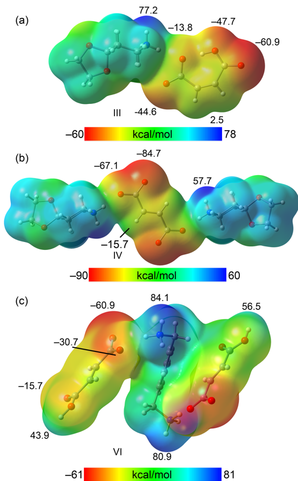
Fig. 22 MEP surfaces of the salts of compounds III, IV and VI. Energies at selected points are indicated. Isosurface 0.001 a.u.
