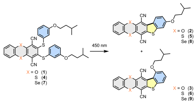
Fig. 1 Structural formulas of chalcogen bridged thioethers and dibenzothioiophenes investigated in this study.
