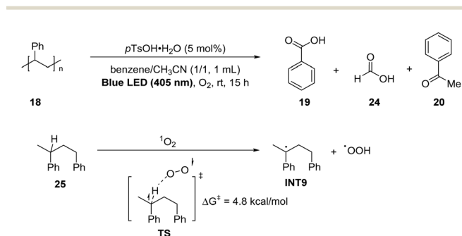
Scheme 9 Acid-catalysed aerobic degradation of polystyrene under visible light.
