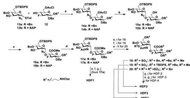
Scheme 1 Synthesis of glucuronic acid based HS disaccharides: (a) NIS, TMSOTf, DCM, -78^\circ\text{C} , 15 min; (b) thiourea, Py: MeOH (1:1), 80^\circ\text{C} , 2 h; (c) (i) TEMPO, BAIB, DCM: \text{H}_2\text{O} (1:1), RT; (ii) MeI, \text{K}_2\text{CO}_3 , DMF, 6 h, RT; (d) Zn dust, THF: AcOH: \text{Ac}_2\text{O} (3:2:1), RT, 12 h; (e) HF.Py, Py, 0^\circ\text{C} , 12 h; (f) DDQ, DCM: \text{H}_2\text{O} (18:1), RT, 1 h; (g) LiOH, \text{H}_2\text{O} : THF (1:1), RT, 12 h; (h) BnBr, \text{NaHCO}_3 , DMF, 60^\circ\text{C} , 2 h; (i) \text{SO}_3\text{-Et}_3\text{N} , DMF, 60^\circ\text{C} , 48–72 h; and (j) \text{H}_2 , \text{Pd}(\text{OH})_2 , \text{H}_2\text{O} , RT, 48 h.
