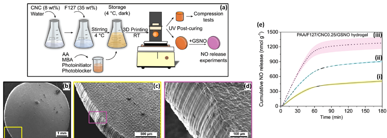
Fig. 7 (a) Scheme of the preparation of 3D printable hydrogel ink comprised of poly(acrylic acid) (PAA), Pluronic F127 micelles (F127), and cellulose nanocrystals (CNC) for DLP 3D printing, followed by S -nitrosoglutathione (GSNO) charging through absorption from solution. (b–d) Representative scanning electron micrographs with increasing magnifications of the surface of 3D-printed PAA/F127/CNC0.25/GSNO hydrogel disks. (e) Real-time NO release from 3D-printed PAA/F127/CNC0.25/GSNO hydrogel discs loaded with GSNO solutions (i) 5 mM, (ii) 10 mM, and (iii) 20 mM. Reprinted (adapted) with permission from M. I. Santos, L. C. E. da Silva, M. P. Bomediano, D. M. Catori, M. C. Gonçalves and M. G. de Oliveira, Soft Matter , 2021, 17, 6352–6361. Copyright 2021.
