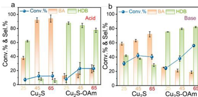
Figure 5. BZH conversion and selectivity toward BA and HDB after 20 min reaction on Cu 2 S and Cu 2 S-OAm electrodes at -0.8 vs. RHE, 25 °C, 45 °C or 65 °C in (a) 1 M sodium acetate-acetic acid solution (pH=5.2) with 20 mM BZH; (b) 1 M potassium carbonate-potassium bicarbonate solution (pH=9.0) with 20 mM BZH.
