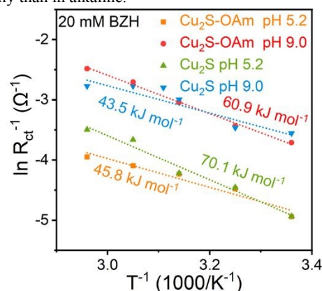
Figure 6. Activation energies calculated from the Nyquist plot.
