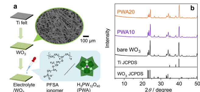
Fig. 1 (a) Preparation of porous \text{WO}_3 photoanode and surface electrolyte coating. (b) XRD patterns of PWA/ \text{WO}_3 photoanodes and the standard lines of \text{WO}_3 (JCPDS No. 01-072-0677) and Ti (JCPDS No. 00-044-1294).
