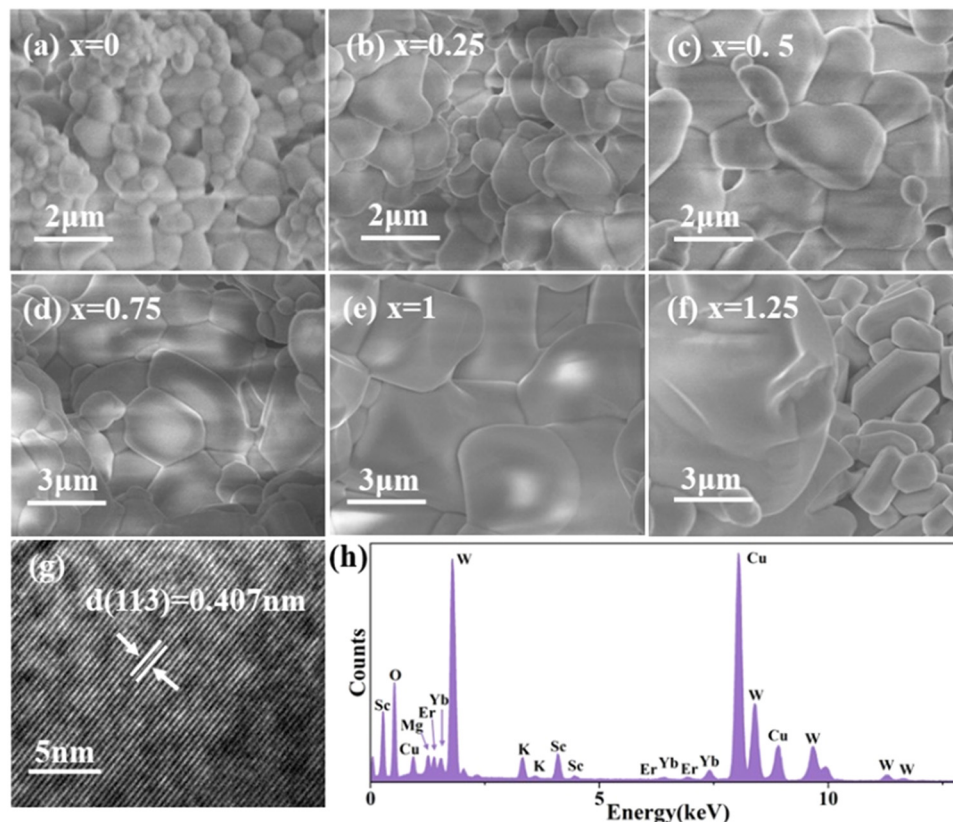
Fig. 3 (a)–(f) SEM images of (\text{KMg})_{1-x}\text{Sc}_x\text{W}_3\text{O}_{12}:1 \text{ mol\% Er}^{3+}/20 \text{ mol\% Yb}^{3+} ( x = 0, 0.25, 0.5, 1, 0.75 , and 1.25 ) phosphors. (g) HRTEM image and (h) EDX results of the (\text{KMg})\text{ScW}_3\text{O}_{12}:1 \text{ mol\% Er}^{3+}/20 \text{ mol\% Yb}^{3+} phosphor.
