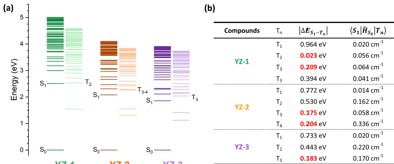
Fig. 6 Results of the TD-DFT calculations at the B3LYP/6-31G** level of theory. (a) Calculated energy level of the singlet and triplet excited states for YZ-1, YZ-2 and YZ-3. (b) Table summarising the results of the TD-DFT calculations of the triplet energy levels including the difference in energy from the S_1 and the spin-orbit coupling value for the transition from S_1 to the corresponding triplet level. To help the eye, the triplet energy levels within ca. \pm 0.2 eV have been highlighted in red. Spin orbit coupling has been calculated using the ORCA software package.
