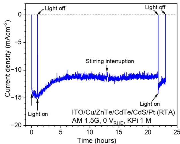
Fig. 9 Time course of the photocurrent generated by an ITO/Cu/ZnTe/CdTe/CdS/Pt photocathode at 0 V_{\text{RHE}} under simulated sunlight in 1 M KPi aqueous solution under 400 rpm stirring.
