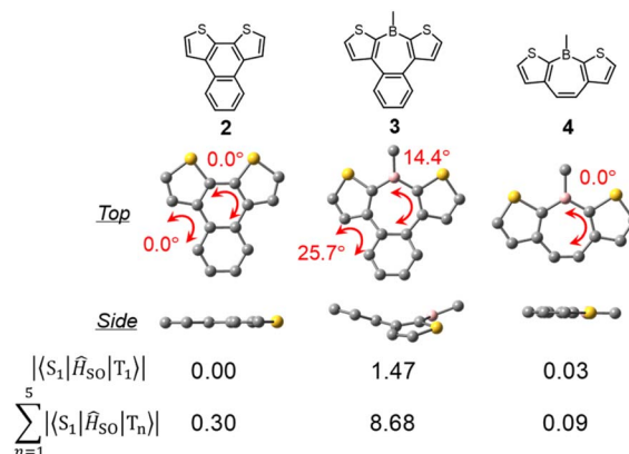
Fig. 8 DFT-optimized S 0 geometries of model compounds and their SOCMEs in cm -1 .
