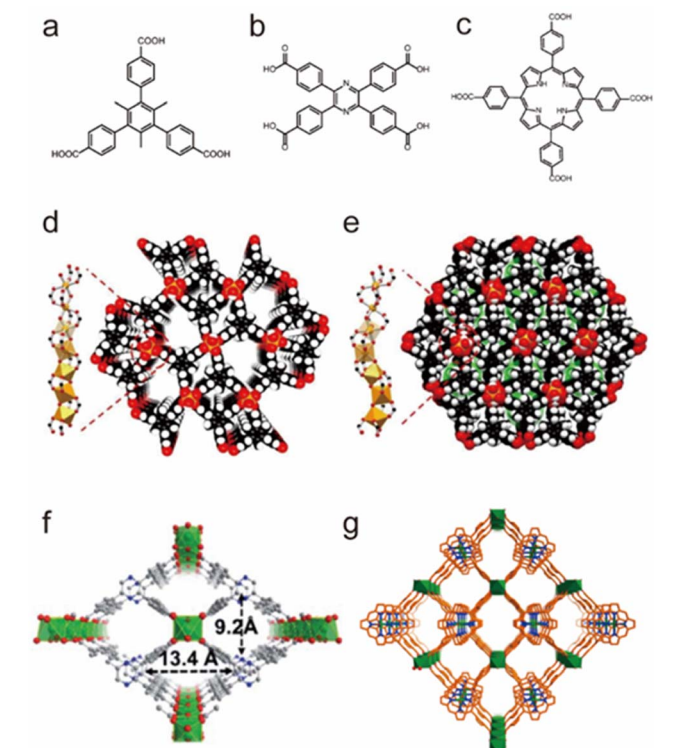
Fig. 6 The structures of representative In(III) -MOFs and the used ligands. (a) The H_3CTTA ligand. (b) The H_4TCPP ligand. (c) The H_2TCPP ligand. (d) BUT-172. Reproduced from ref. 103 with permission from the Royal Society of Chemistry, Copyright 2020. (e) BUT-173. Reproduced from ref. 103 with permission from the Royal Society of Chemistry, Copyright 2020. (f) In(tcpp) . Reproduced from ref. 104 with permission from the Royal Society of Chemistry, Copyright 2021. (g) USTC-8. Reproduced from ref. 105 with permission from the American Chemical Society, Copyright 2018.
