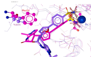
4-(5-(1-Isopropyl-6-oxo-4,5,6,7-tetrahydro-1H-pyrazolo[3,4-b]pyridin-4-yl)furan-2-yl)benzenesulfonamide
