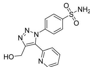
4-(4-(Hydroxymethyl)-5-(pyridin-2-yl)-1H-1,2,3-triazol-1-yl)benzenesulfonamide
