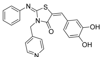
(E)-5-((E)-3,4-Dihydroxybenzylidene)-2-(phenylimino)-3-(pyridin-4-ylmethyl)thiazolidin-4-one
