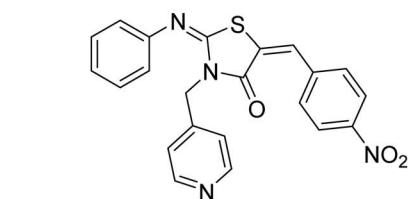
(E)-5-((E)-4-Nitrobenzylidene)-2-(phenylimino)-3-(pyridin-4-ylmethyl)thiazolidin-4-one
