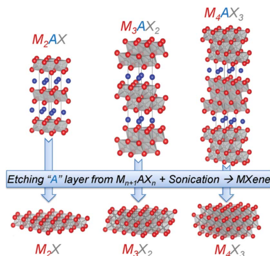
Fig. 1 Structures of MAX phases and their derived pristine MXene nanosheets. M is a transition metal, e.g. , Ti; A is an element from group 13 or 14, e.g. , Al. X is C, N, or their combination. 24 Copyright 2013, Wiley-VCH.
