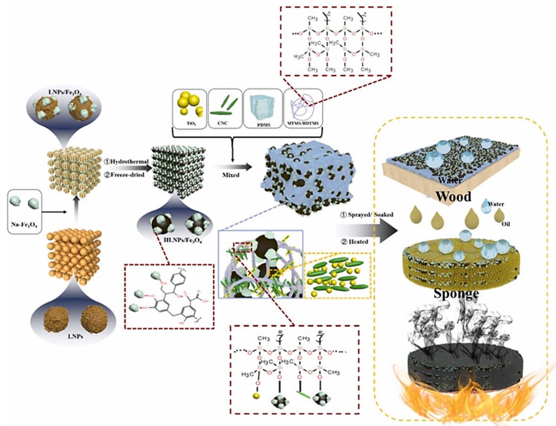
Fig. 14 Diagram illustrating the superhydrophobic coating's fabrication procedure using HLNs and \text{Fe}_3\text{O}_4 . 102 Reproduced from ref. 102 with permission from Journal of Environmental Chemical Engineering , copyright 2023.
