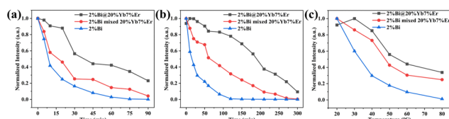
Fig. 5 Comparison of the PL intensity of 2%Bi@20%Yb, 7%Er core-shell NCs, the mixture of 2%Bi NCs and 20%Yb, 7%Er NCs and 2%Bi NCs under 370 nm excitation: (a) in cyclohexane and DI water ( v/v = 1:9 ) mixed solvents under 370 nm excitation; (b) under continuous UV light irradiation; (c) at different temperatures.
