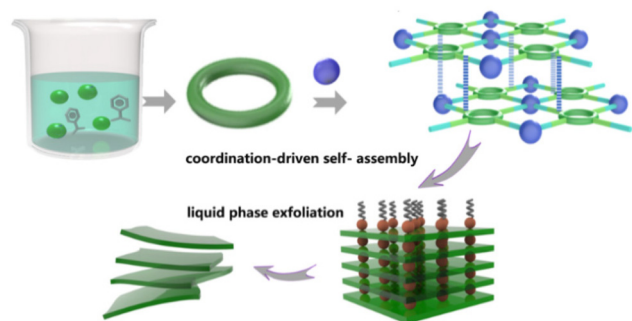
Scheme 1 Schematic diagram showing the stepwise designed synthesis of the layer compound based on the aluminum molecular ring and the liquid phase exfoliation for nanosheets.
