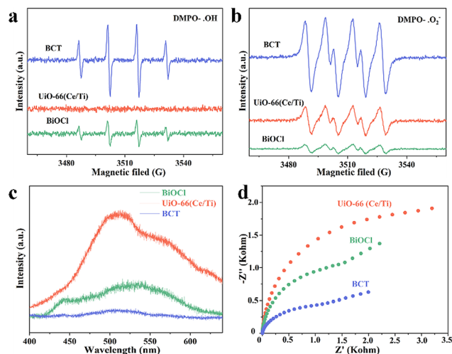
Fig. 6 Electron paramagnetic resonance (EPR) spectra of (a) DMPO–OH adducts and (b) DMPO–O 2 − adducts over BiOCl, UiO-66(Ce/Ti), and BCT under illumination for 2 min. (c) Steady-state photoluminescence (PL) spectra and (d) electrochemical impedance spectroscopy (EIS) spectra of BiOCl, UiO-66(Ce/Ti), and BCT.
