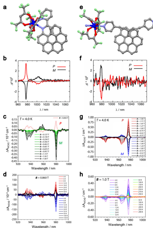
Fig. 3 Molecular structure of (P)6-Yb (a) and [(P)7-Yb] n (e); H atoms and solvent molecules of crystallization were omitted for clarity. Grey, C; red, O; blue, N and dark blue, Yb. CPL spectra (at 298 K) of (P)6-Yb (red line)/(M)6-Yb (black line) (b) and [(P)7-Yb] n (red line)/(M)7-Yb (black line) (f) under 365 nm excitation in solid-state. Field dependence of the difference in the absorption \Delta A_{MChD} of the ^2F_{7/2} \rightarrow ^2F_{5/2} transition at 4 K for (P)6-Yb (c) and [(P)7-Yb] n (g). Thermal dependence of the difference in the absorption \Delta A_{MChD} of the ^2F_{7/2} \rightarrow ^2F_{5/2} transition for (P)6-Yb under 0.86 T (d) and [(P)7-Yb] n under 1 T (h). Adapted with permission from ref. 23 and 25. Copyright 2021, American Chemical Society. Copyright 2023, Wiley-VCH Verlag GmbH & Co. KGaA Weinheim.
