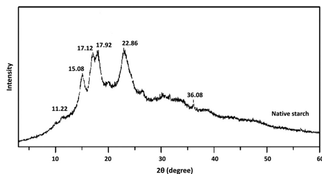
Fig. 3 X-Ray diffraction pattern of native cassava starch. Native cassava starch exhibits three strong diffraction peaks ( 2\theta ) at 15.08°, 17.92°, and 22.86°, which indicates a type A crystalline structure. Adapted from open access article under Creative Commons license: Yi et al., 2020. 56
