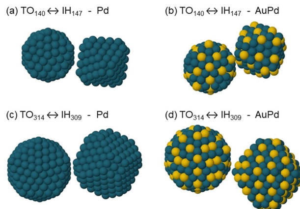
Fig. 1 Initial configurations for the molecular dynamics simulations of the TO ↔ IH coalescence. (a) Coalescence of a TO cluster of 140 atoms and an IH of 147 atoms, with pure Pd composition. (b) Same structures and sizes as in (a), but with ~20% of Au atoms. (c) Coalescence of a TO cluster of 314 atoms and an IH of 309 atoms, with pure Pd composition. (d) Same structures and sizes as in (c), but with ~20% of Au atoms. The colliding units are 3–4 Å apart, with random mutual orientation. In (b) and (c), all Au atoms are in the nanoparticle surfaces, in the most favourable placement according to basin hopping calculations.
