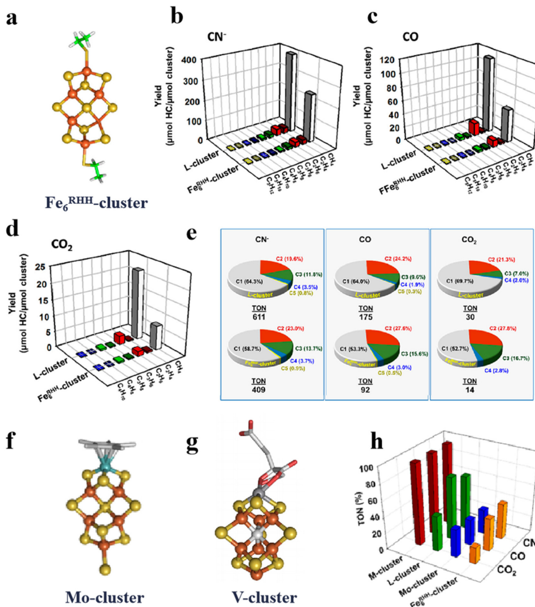
Fig. 6 Artificial Fe-S clusters based on configuration design to improve catalytic performance. (a) Structure of \text{Fe}_6^{\text{RHH}} -cluster. Types and yields of L- and \text{Fe}_6^{\text{RHH}} -clusters for the reduction of (b) \text{CN}^- , (c) CO and (d) \text{CO}_2 to hydrocarbons. (e) L- and \text{Fe}_6^{\text{RHH}} -clusters percentage of products forming hydrocarbons. (f) Structure of Mo-cluster. (g) Structure of V-cluster. (h) TON of M-, L-, Mo- and \text{Fe}_6^{\text{RHH}} -clusters for the reduction of \text{CN}^- , CO and \text{CO}_2 . Reproduced with permission from ref. 36. Copyright 2017, American Chemical Society.
