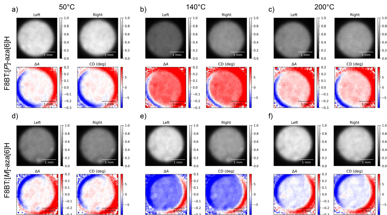
Fig. 2 Circular dichroism images of 140 nm thick solid state F8BT:[P]-aza[6]H (a, b, c) and F8BT:[M]-aza[6]H (d, e, f) films at annealing temperatures of 50^\circ\text{C} (a, d), 140^\circ\text{C} (b, e), and 200^\circ\text{C} (c, f) taken using the two camera circular dichroism imaging system at a wavelength of 470 nm. In each subfigure, “Left” and “Right” indicate the transmitted intensities of L-CPL and R-CPL (respectively), \Delta A is calculated using eqn (5) and “CD” is the degrees of ellipticity calculated using eqn (2).
