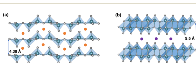
Fig. 4 Pre-intercalated \alpha - V_2O_5 into (a) “hinged” structure and (b) bilayered structures with expanded interlayer distance. Reproduced with adaption from ref. 58 with permission from Elsevier. Copyright 2019.
