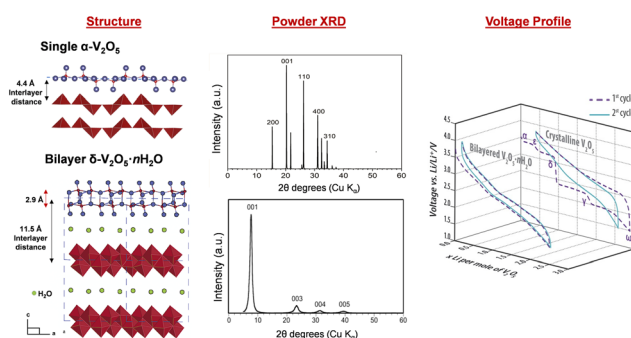
Fig. 7 Structural and electrochemical comparison between crystalline V_2O_5 and bilayered \delta-V_2O_5 \cdot nH_2O . Reproduced and adapted from ref. 23, 102 and 103, with permission from Elsevier, copyright 1994, John Wiley & Sons, copyright 2016, American Chemical Society, copyright 2002.
