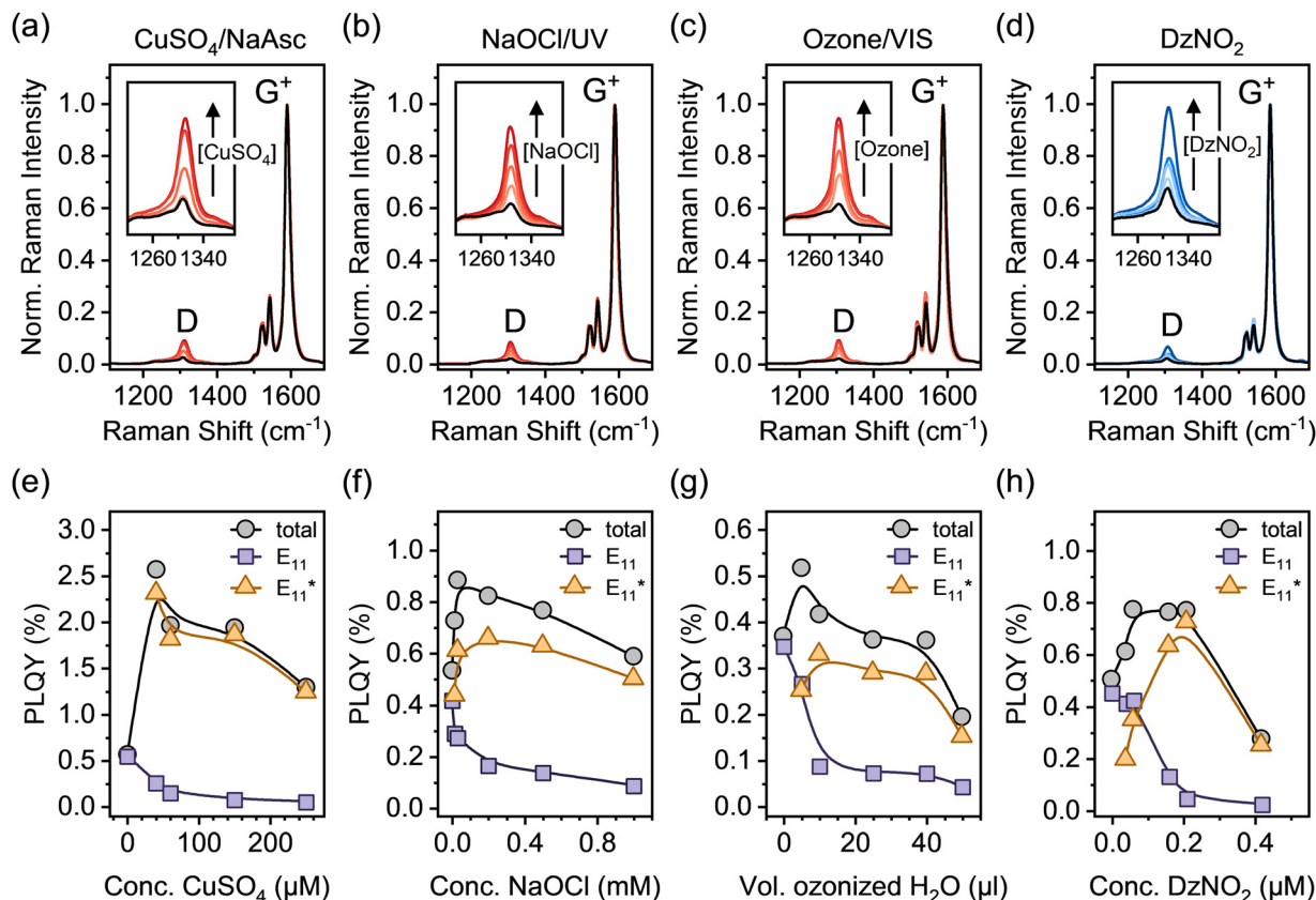
Fig. 2 (a)–(d) Normalized (to G + peak) averaged Raman spectra of pristine (black) and different functionalized (6,5) SWCNTs ( \lambda_{\text{exc}} = 532 nm, >3600 individual spectra for each sample). The insets show the evolution of the defect-related D-mode with increasing degree of functionalization. (e)–(h) Corresponding total and spectrally resolved PLQYs for pristine and different functionalized (6,5) SWCNTs in aqueous dispersion depending on reactant concentration (after surfactant exchange to 1% (w/v) DOC).
