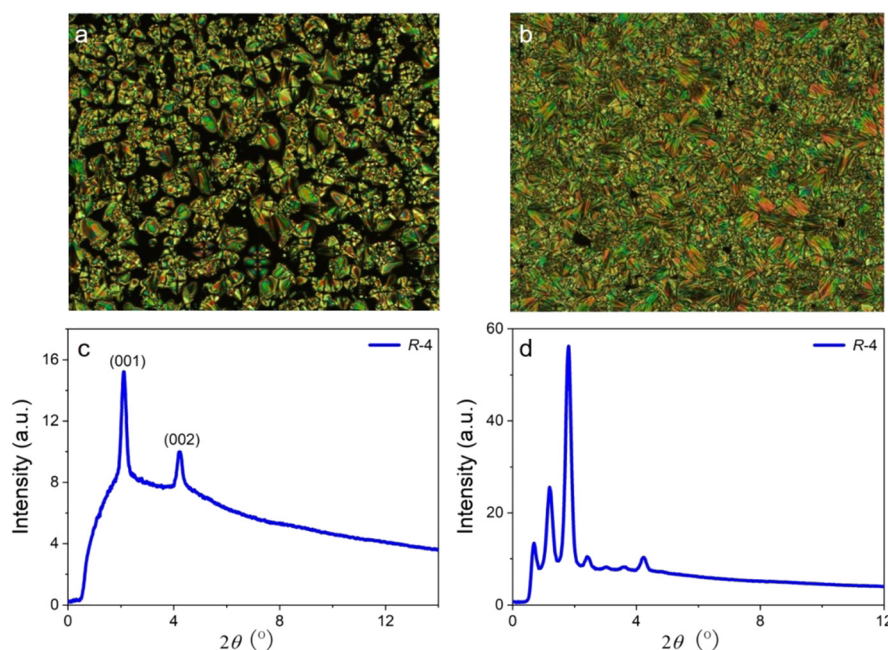
Fig. 3 POM image of R-4 on cooling: (a) in the SmA^* phase at 183 °C and (b) in the more ordered mesophase at 155 °C. SAXS pattern of R-4 on cooling: (c) in the SmA^* phase at 173 °C and (d) in the more ordered mesophase at 148.4 °C.
