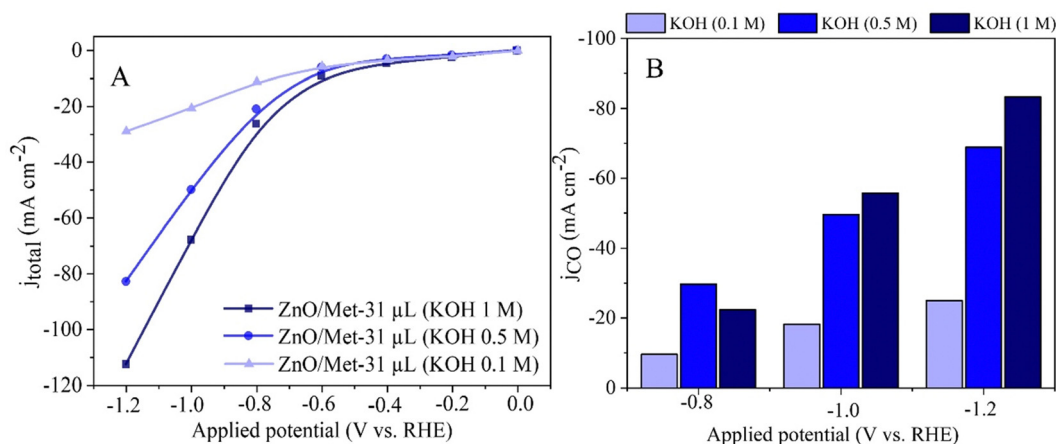
Fig. 8 (A) Polarization curves of the ZnO/Met-31 \mu\text{L} under different concentrations of KOH electrolyte. (B) The partial current density for CO ( j_{\text{CO}} ) formation in different concentrations of KOH.
