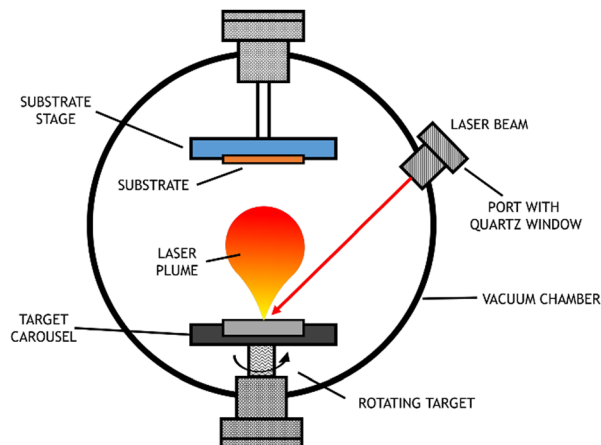
Fig. 7 Scheme of pulsed laser deposition equipment.
