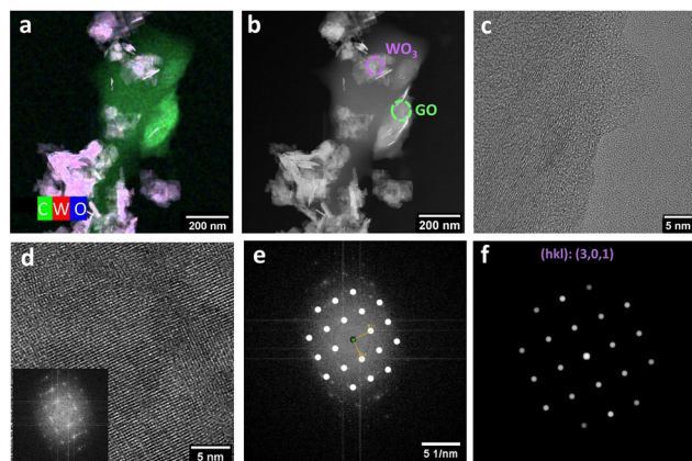
Fig. 5 (a) HAADF-STEM micrograph of \text{WO}_3\text{GO}_{200\text{ °C-10 min}} with the elemental map obtained from \text{W}_{\text{L}\alpha} , \text{O}_{\text{K}\alpha} , and \text{C}_{\text{K}\alpha} . (b) HAADF image with selected regions of \text{WO}_3 and GO and (c) HRTEM images of GO and (d) \text{WO}_3 with a fast-Fourier-transform pattern (FFT – inset). (e) FFT pattern fitted with the schematic diagram of monoclinic \text{WO}_3 (301) and (f) calculated diffraction pattern (301).
