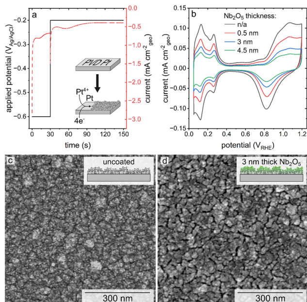
Fig. 1 (a) Current density and potential recorded as a function of time during the sequential, double pulse electrodeposition of a textured Pt catalyst. (b) A series of cyclic voltammetry plots corresponding to the textured Pt catalysts (both without and with niobia or Nb 2 O 5 coatings as indicated in the legend) before an accelerated stress test (AST). Scanning electron microscopy (SEM) images of pristine Pt with a nanoscale texture (c) and the same substrate after coating with a 3 nm thick layer of Nb 2 O 5 (d).
