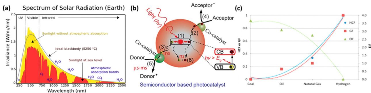
Fig. 4 (a) Illustration of the solar spectrum and absorption by atmospheric gases in the wavelength range of 240 nm to 2.5 μm. 77 Reproduced with permission from ref. 77 Copyright via Wikimedia Commons. (b) Fundamental operating mechanisms of semiconductor-based photocatalysts. 78 Reproduced with permission from ref. 78 Copyright © 2022 Tsinghua University Press Ltd. (c) Comparison of Hydrogen Combustion Efficiency (HCF), Greenhouse Gas Footprint (GF), and Energy Intensity Factor (EIF) between hydrogen and other fossil fuels. 81 Reproduced with permission from ref. 81 Copyright © 2014 Hydrogen Energy Publications, LLC. Published by Elsevier Ltd. All rights reserved.
