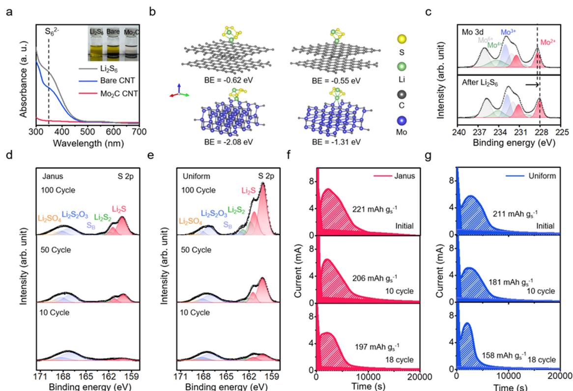
Fig. 3 Suppression of LiPS shuttle in the Janus film cathode. (a) UV-vis absorption spectra of bare and Mo 2 C-CNT immersed in Li 2 S 6 electrolyte. The inset image shows the color change after adsorption. (b) Optimized adsorption configurations and binding energies on carbon and Mo 2 C surfaces for Li 2 S 6 and individually for Li 2 S 4 . (c) Mo 3d XPS spectra of the Mo 2 C-CNT substrate before and after the adsorption of Li 2 S 6 . Ex situ XPS spectra of the Li metal anode (d) in Janus film cathode cells during charge/discharge cycles and (e) in uniform film cathode cells. Galvanostatic discharge profiles for the LiPS-Li 2 S conversion during charge/discharge cycles in (f) Janus film cathode cells and (g) in uniform film cathode cells.
