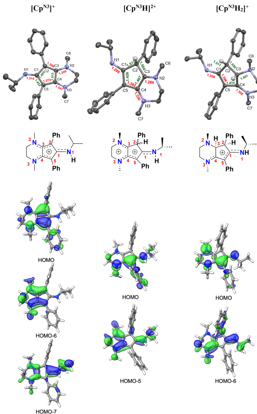
Fig. 6 Top: X-ray crystallographic structures of [Cp^{N^3}][B(C_6F_5)_4] (left), [Cp^{N^3H}][BF_4]_2 ( [4][BF_4]_2 , middle), and [Cp^{N^3H_2}][PF_6] ( [5][PF_6] ; right) with 50% probability ellipsoids. Co-crystallized solvent molecules, counterions, and most hydrogens have been omitted for clarity. Middle: structural cartoons showing charge delocalization based on metrical parameters and typical interatomic distances for organic compounds (see Table 1 and discussion). Bottom: selected molecular orbitals for all three molecules, showing the main \pi -type MOs responsible for electron delocalization involving the Cp ring (isovalue = 0.04).
