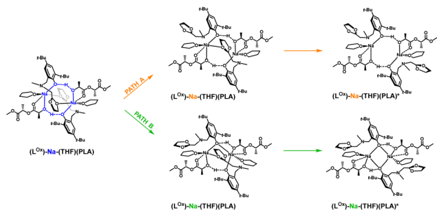
Fig. 14 Proposed version of the active catalyst (L^{Ox})\text{-Na-(THF)(PLA)} structural motif with decooordination of amine arms in the degradation reaction of PLA.
