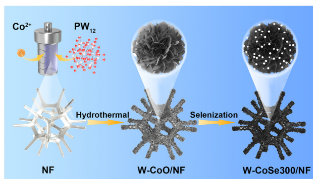
Fig. 1 Schematic diagram of the synthesis process of \text{W-CoSe}_{300}/\text{NF} snowflake flakes.
