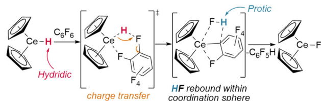
Fig. 11 Calculated mechanism of \text{Cp}^*_{\text{H}}\text{CeH} reactions with \text{C}_6\text{F}_6 (shown as calculated with \text{Cp} (i.e. \text{C}_5\text{H}_5 ) for computational simplicity).
