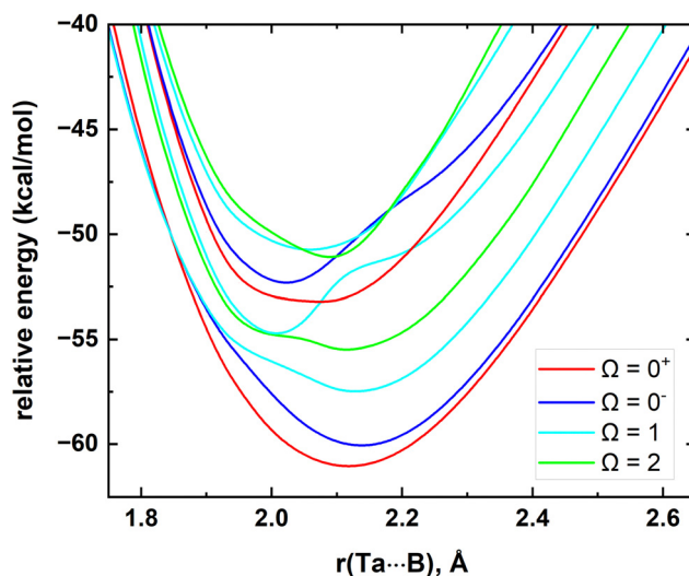
Fig. 3 Low-lying spin-orbit coupling curves of TaB as a function of Ta...B distance [ r(\text{Ta} \cdots \text{B}) , Å]. The relative energies are referenced to the energy of the lowest \Omega state of Ta( 4 F) + B( 2 P) fragments at r = 200 Å, which is set to 0 kcal mol -1 . The \Omega = 0^+ , \Omega = 0^- , \Omega = 1 , and \Omega = 2 curves are shown in red, blue, cyan, and green, respectively.
