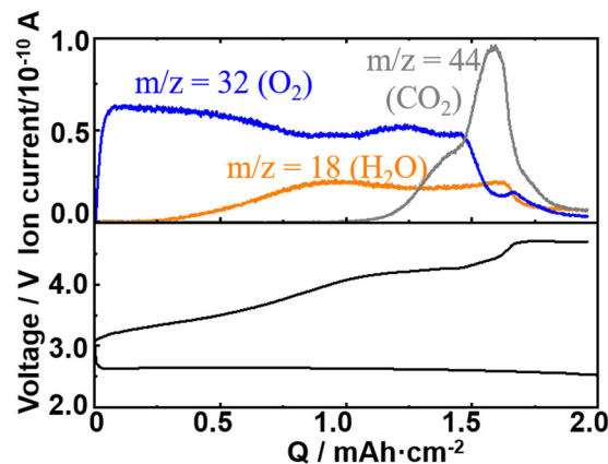
Fig. 2 Typical discharge/charge curves (bottom panel) and ion currents of the Q-mass at m/z = 18 ( H_2O ), 32 ( O_2 ), and 44 ( CO_2 ) during charge (top panel) of a Li/TEGDME-1M LiTFSI/KJCNT cell (electrode area: 2\text{ cm}^2 ) obtained under a constant current of 0.4\text{ mA} ( 0.2\text{ mA cm}^{-2} ).
