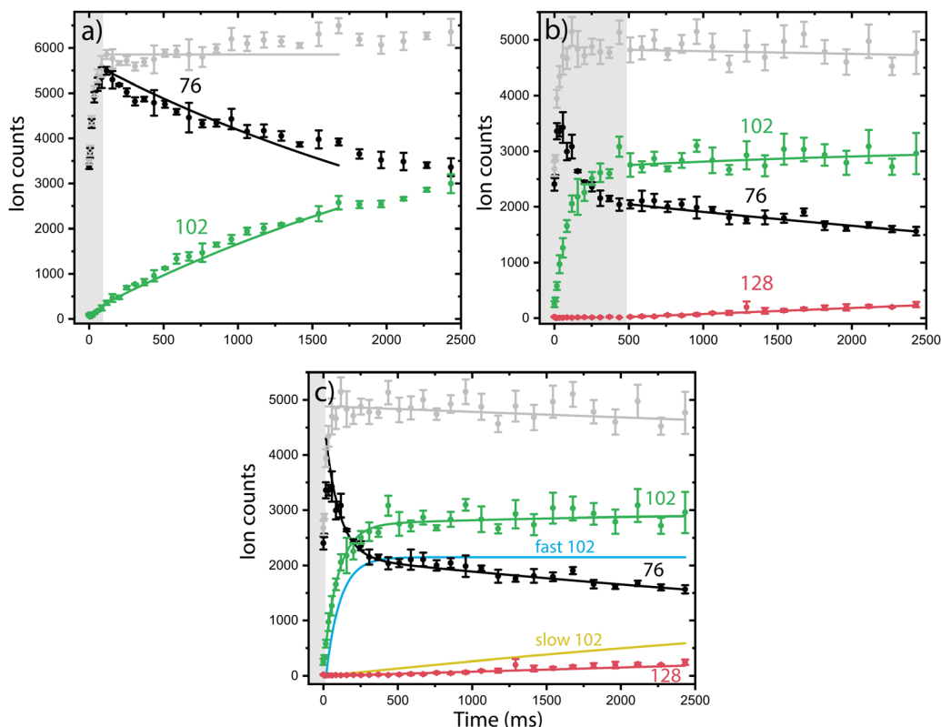
Fig. 3 Representative kinetic plots of the o -benzynes •+ (O)/ m -benzynes •+ (M)/ethynyl–methylene–cyclopropene •+ (E) with acetylene ion–molecule reaction at 150 K for (a) low (1.36(\pm 0.15) \times 10^9 \text{ cm}^{-3}) and (b) and (c) high (2.17(\pm 0.23) \times 10^{10} \text{ cm}^{-3}) acetylene number density. The experimental ion counts of the reactants ( m/z 76, black), intermediate m/z 102 (green) and product structure m/z 128 (red) at different trapping times are plotted with dots and error bars. The data in panel a and b are fitted with the reduced ODE master equation whereas the data in panel c is fitted with the biexponential model (solid lines, explanation see text). The grey box indicates the data points that were not used in the fitting process.
